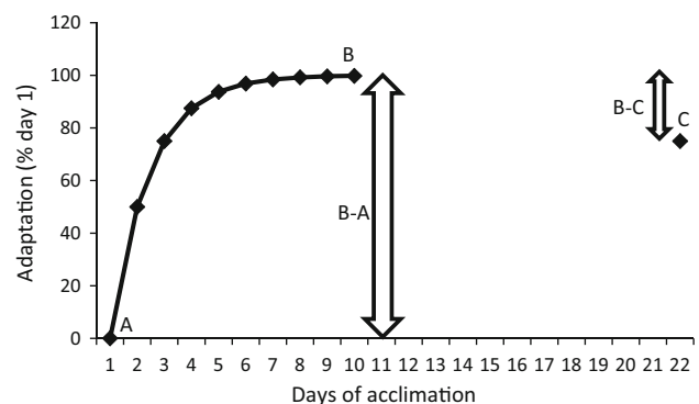
Fig. 2 Example of the heat acclimation decay calculation. A is the heat unacclimated state, B is the acclimated state, and C is the status on return following a decay period without heat exposure (e.g., 12 days after the final day of heat acclimation). % Decay is defined as (B-C)/(B-A)
